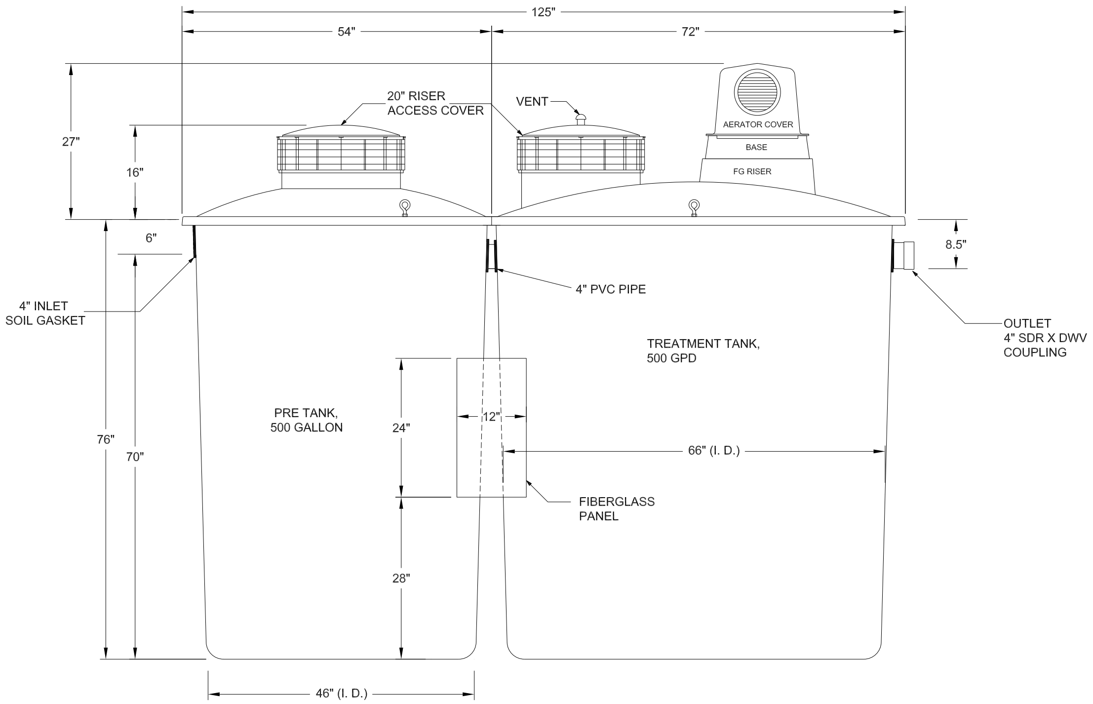
SIDE VIEW
