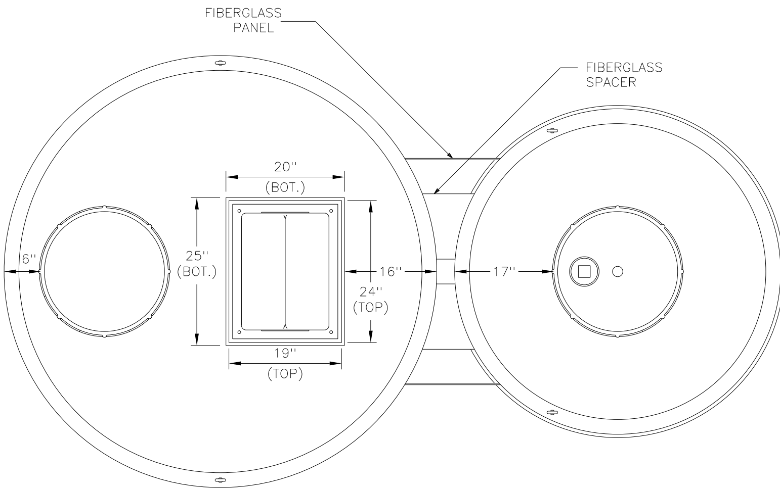
TOP VIEW
