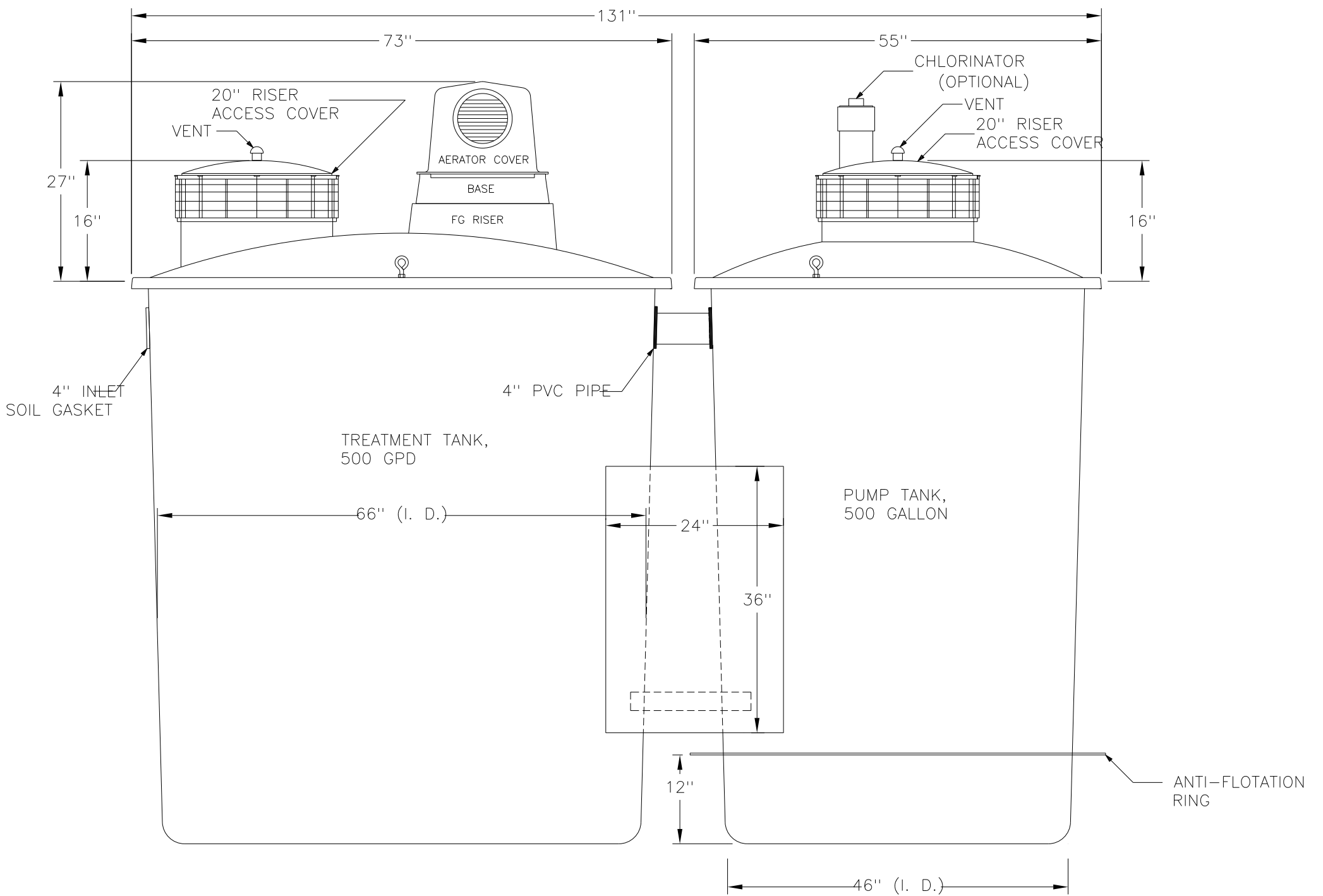
SIDE VIEW
