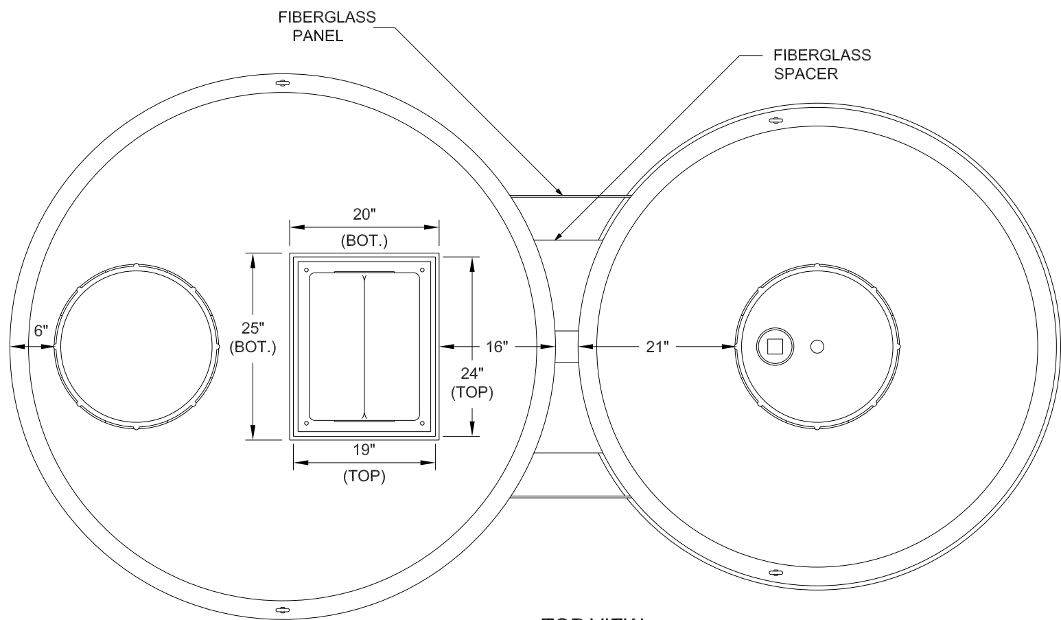
TOP VIEW
