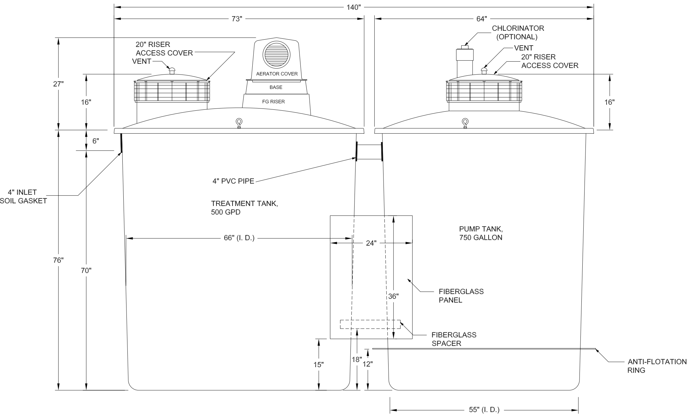
SIDE VIEW
